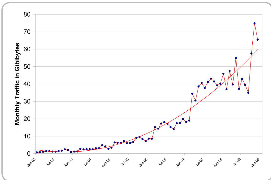
Fig. 1. CAEPR web traffic, Jan 2003–Dec 2008
